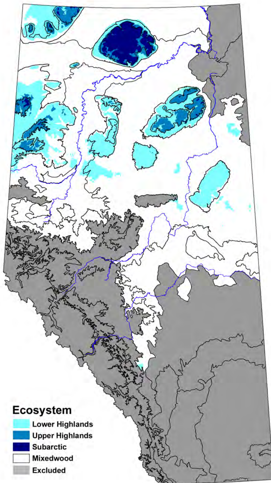
Fig. 3.9. Predicted ecosystems for the Boreal Highlands Bioclimatic Envelope Model, using climate data from the 1961-1990 reference period as input.
