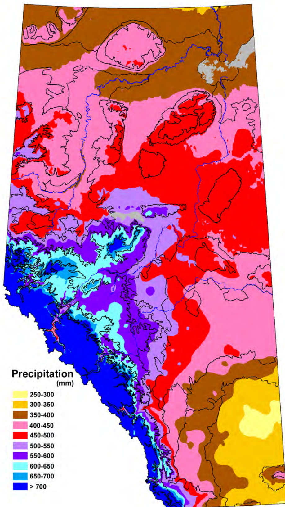
Fig. 3.2. MAP for the 1961-1990 reference period. Natural Subregions are outlined in black.
