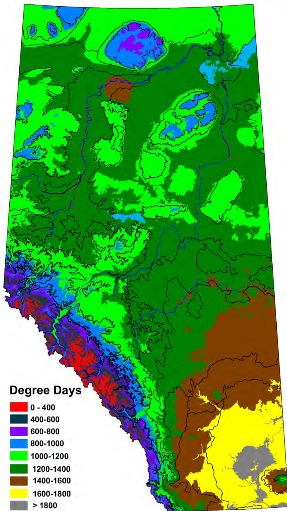
Fig. 3.5. Growing degree-days greater than 5 °C for the 1961-1990 reference period. Natural Subregions are outlined in black.
