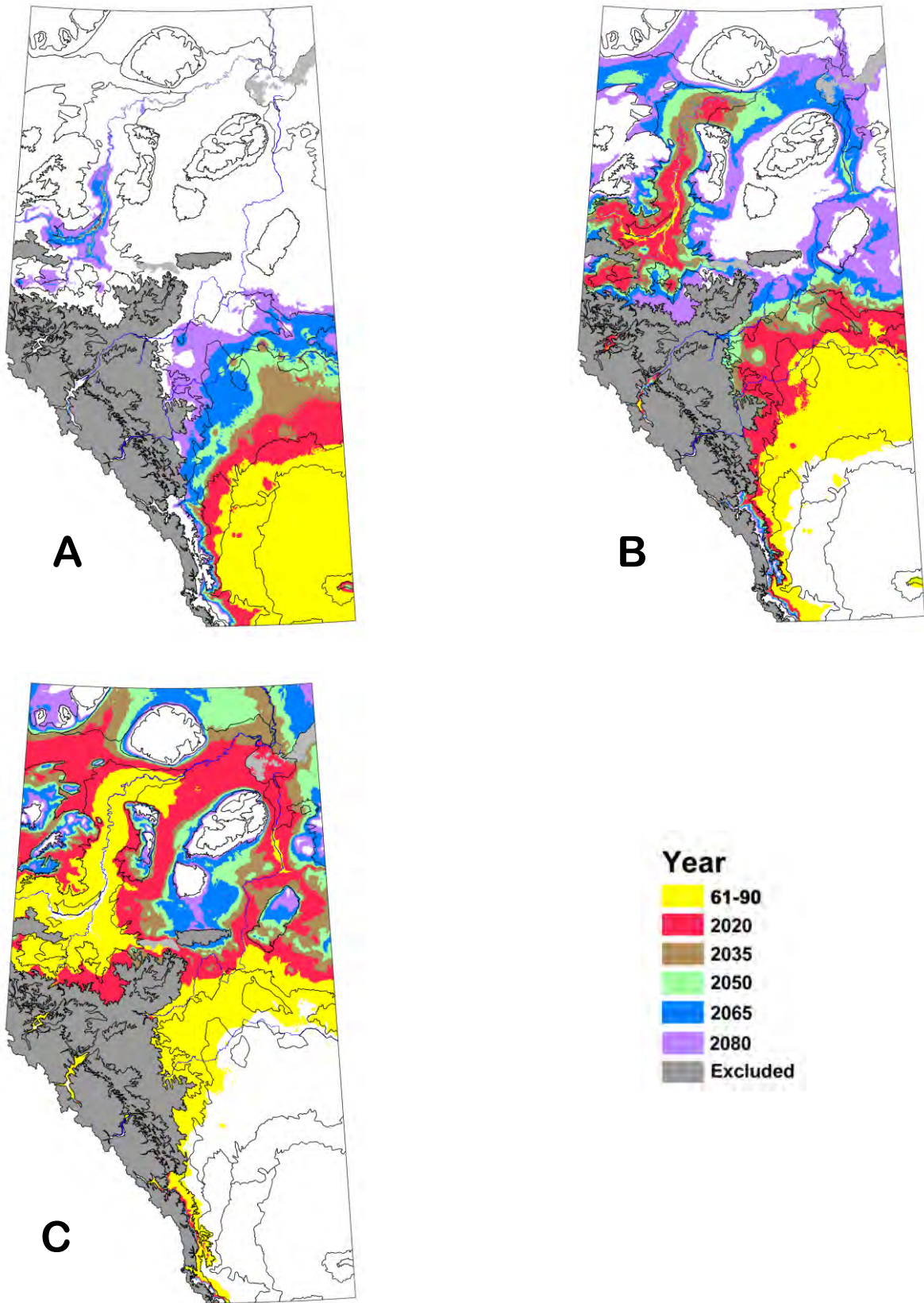
Temporal change in the climate envelopes for the Wet model: Panel A= Grassland; Panel B = Parkland; Panel C = Deciduous Forest.
