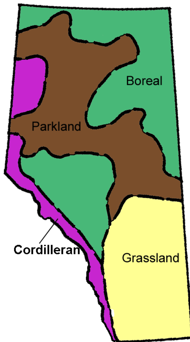
Fig. 2.3. Ecosystem reconstruction for the Hypsithermal period, derived from Strong and Hills, 2005.
