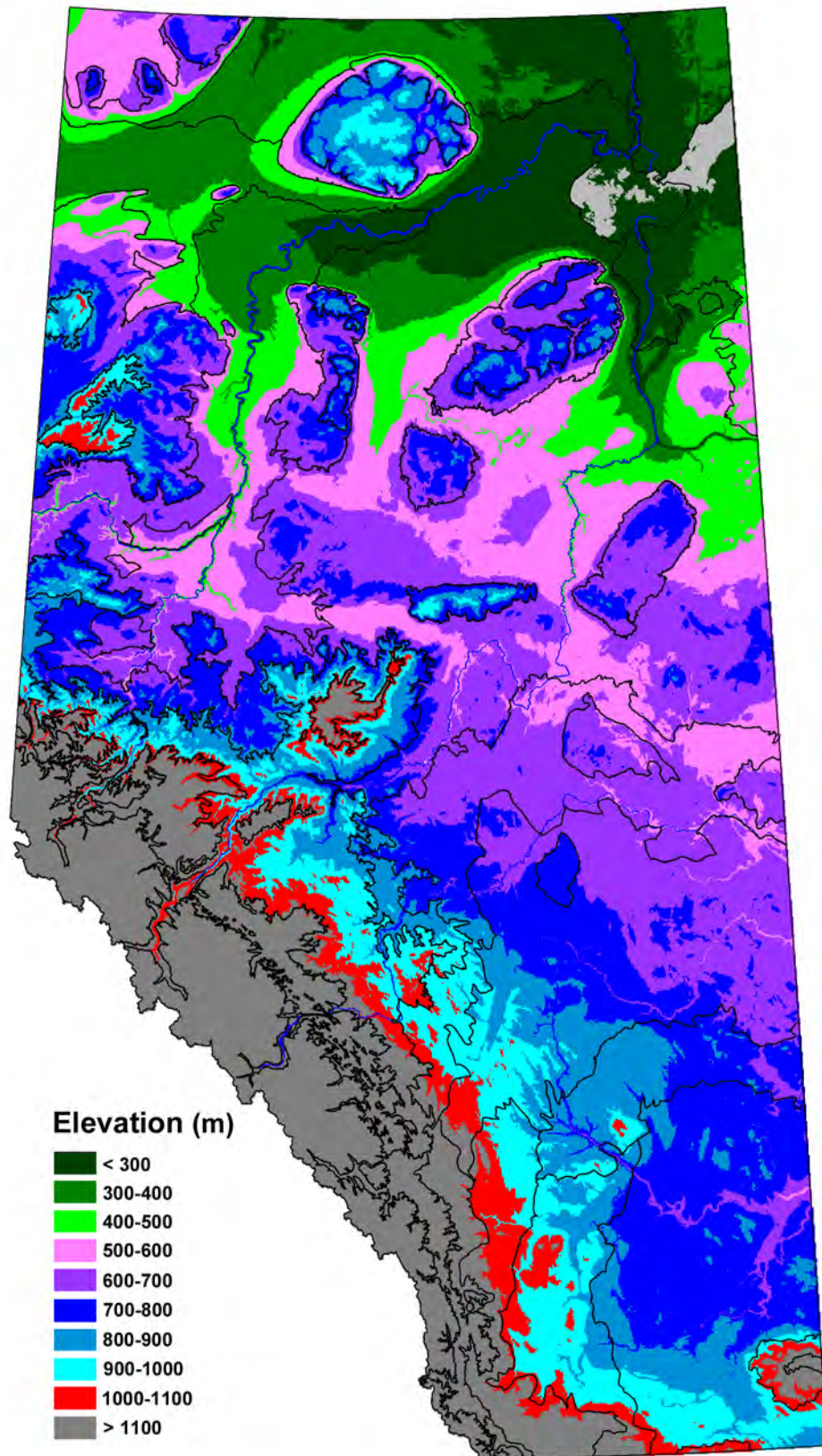
Fig. 3.8. Elevation. Natural Subregions are outlined in black.
