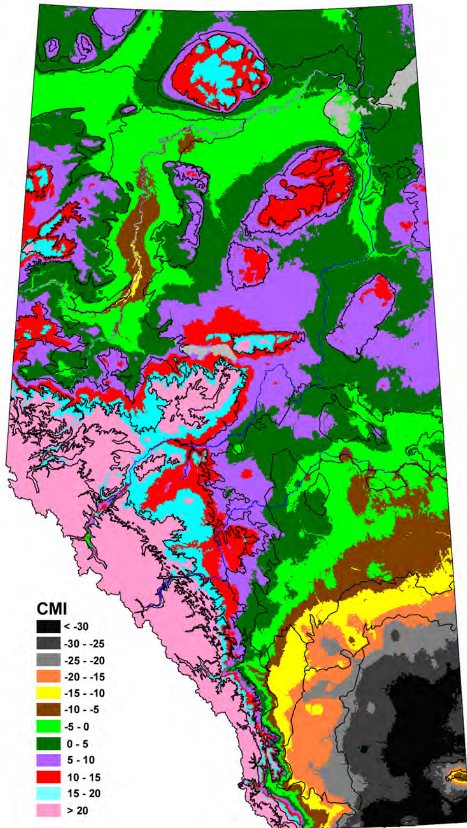
Fig. 3.3. CMI for the 1961-1990 reference period. Natural Subregions are outlined in black.
