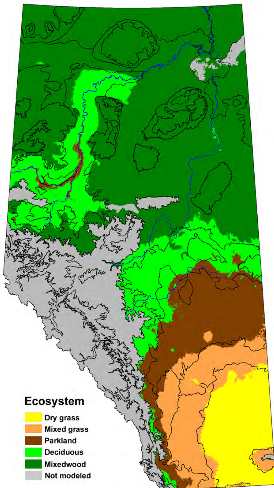
Fig. 3.7. Predicted ecosystems for the Grassland to Boreal Bioclimatic Envelope Model, using climate data from the 1961-1990 reference period as input.
