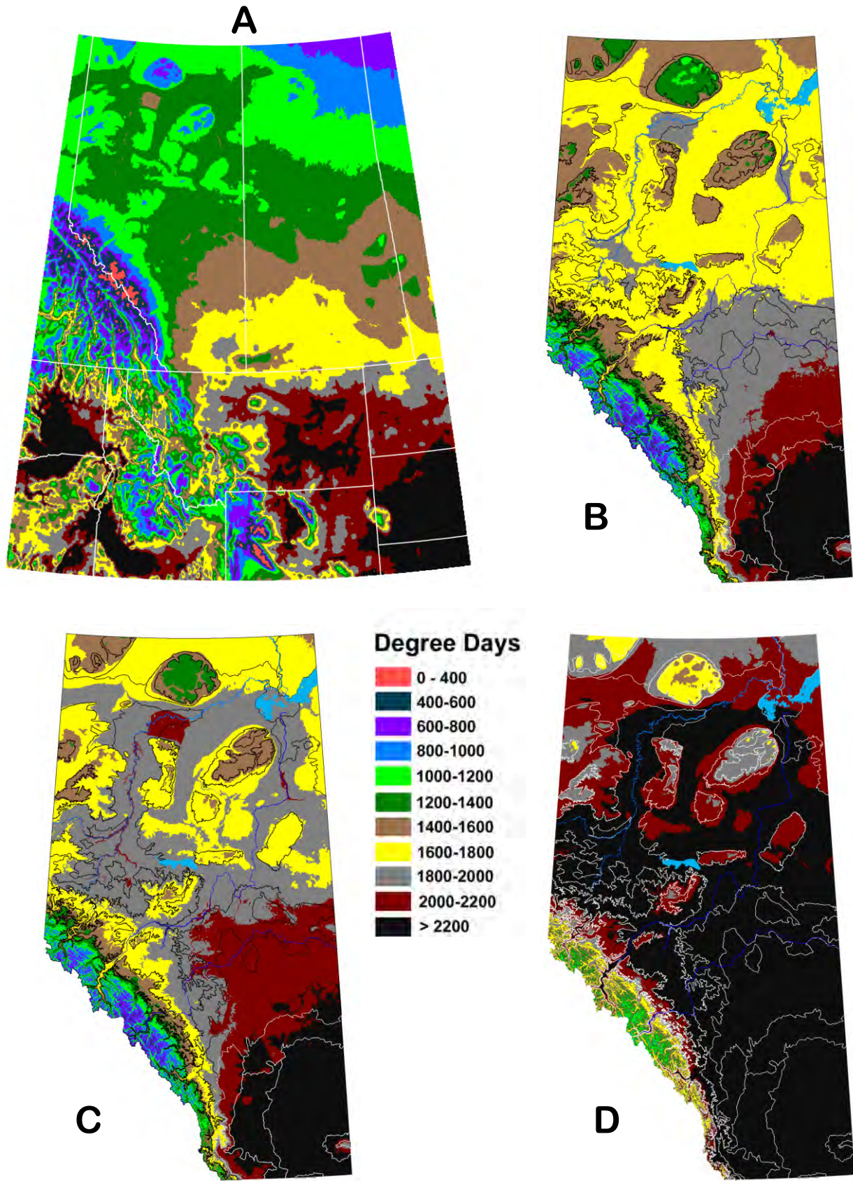
Fig. 4.6. Mean growing degree-days in 1961-1990 (Panel A) and in the 2080s: Panel B = Cool model; Panel C = Median model; Panel D = Hot model.
